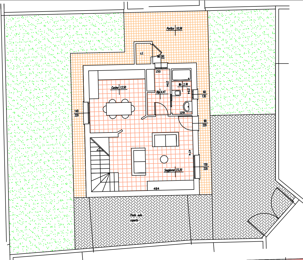
Piano terra
